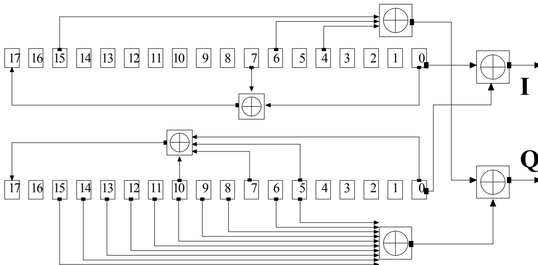
Fig. 4-17 Structure of downlink scrambling code generator
