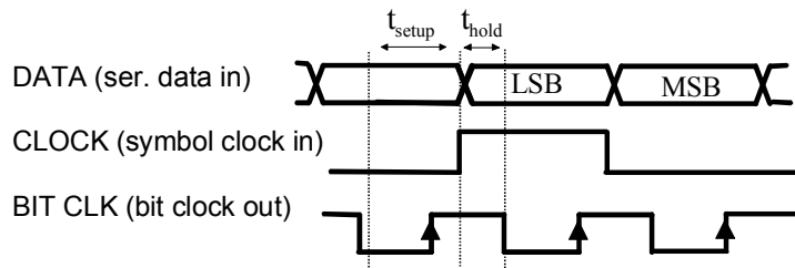
Fig. 4-8 External serial data and external symbol clock - 3 bits/symbol with high and low active symbol clock for marking the LSB. The data and the symbol clock must change state simultaneously. The setup time ( t_{\text{setup}} ) and hold time ( t_{\text{hold}} ) can be found in the data sheet.
