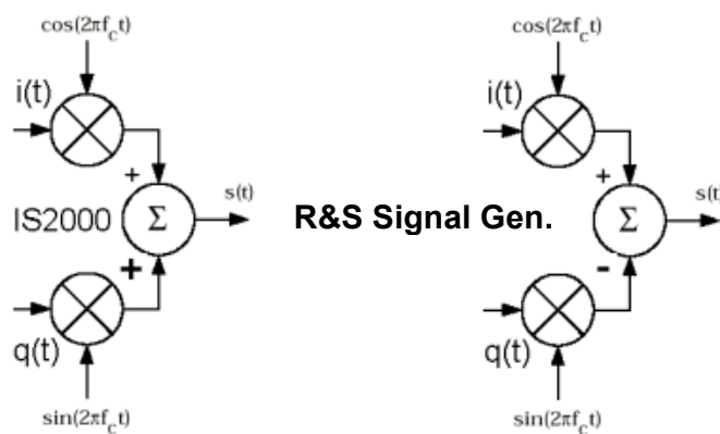
Fig. 4-47 Definition of IQ modulator in IS2000 and R&S Vector Signal Generator
