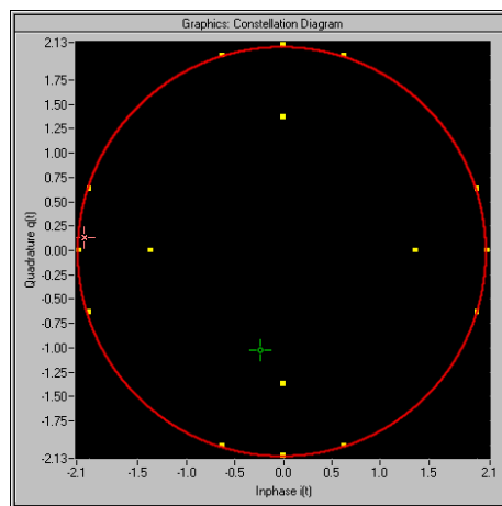
Fig. 4-51 Constellation diagram with clipping level 80 %, vector mode ( |i+q| ) The circle emphasizes the changed constellation points.
