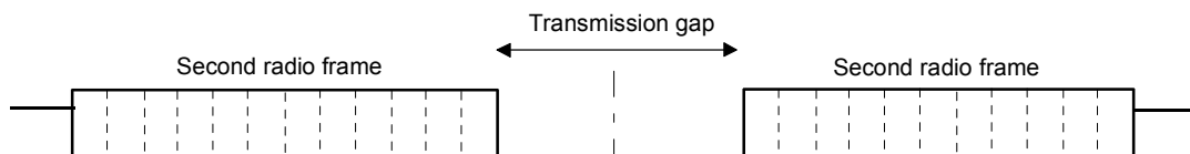
Fig. 4-26 Envelope of compressed mode signal with double-frame method
