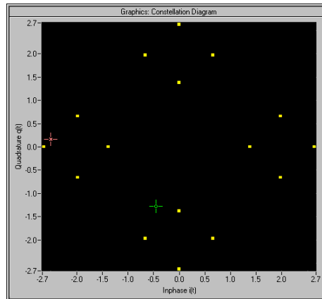
Fig. 4-50 Constellation diagram of the signal without clipping, shows the level mapping
