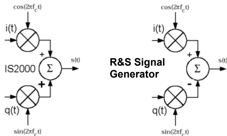
Fig. 4-2 Definition of I/Q modulator in IS2000 and R&S Vector Signal Generator
