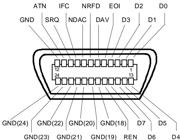
Figure 5-4 Pin assignment of IEC/IEEE-Bus interface
