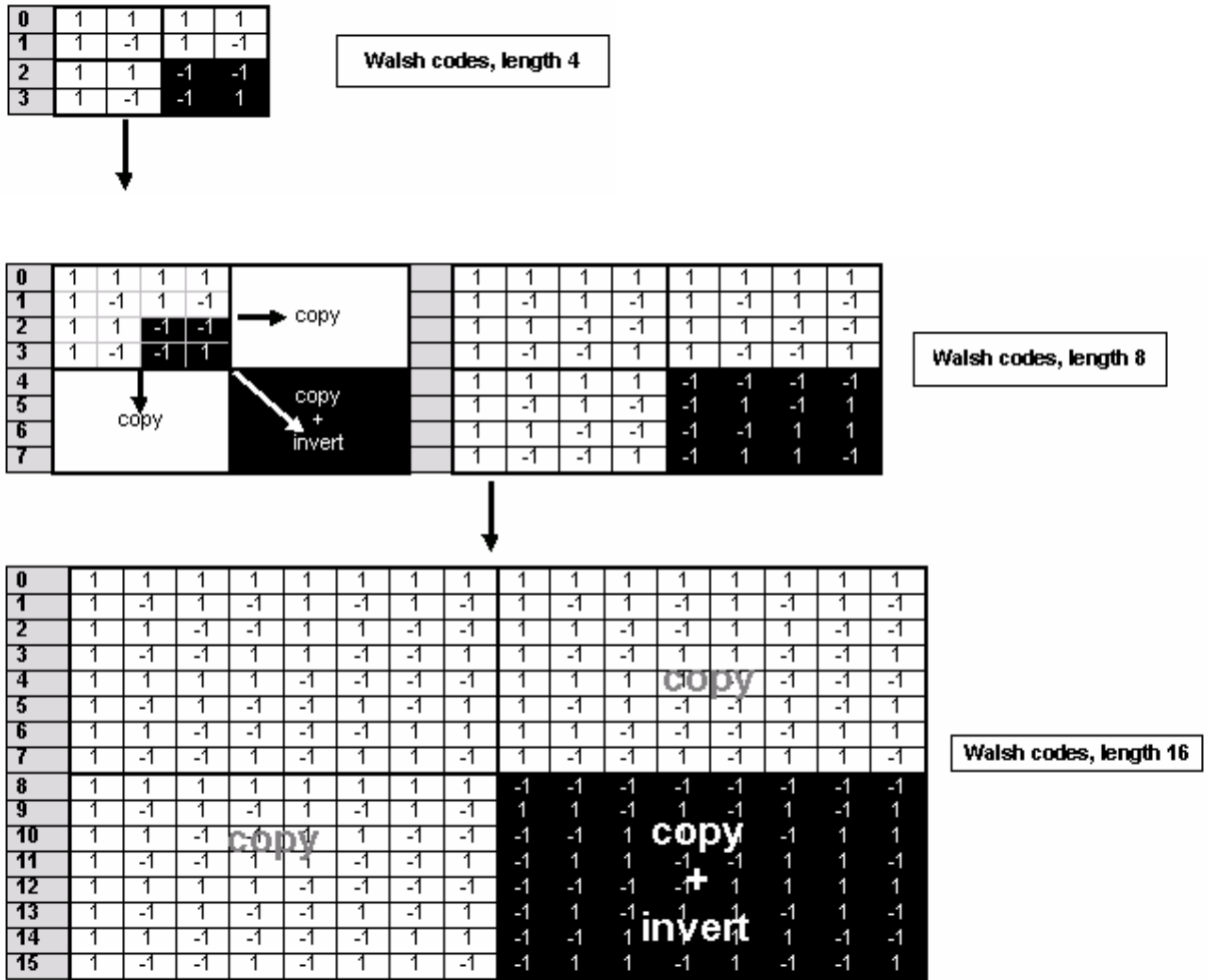
Fig. 4-52 Generation scheme of Walsh code
