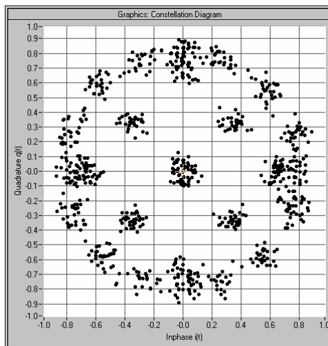
Fig. 4-64 Constellation diagram with clipping level 380 %, vector mode (|i+jq|) .
