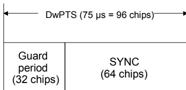
Fig. 4-59 Structure of DwPTS
