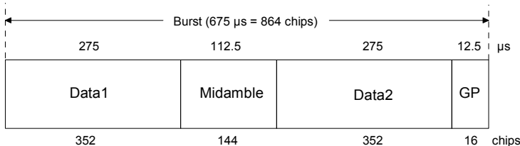
Fig. 4-61 Traffic burst without layer 1 control information
