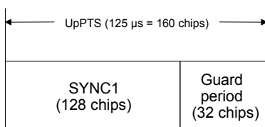
Fig. 4-60 Structure of UpPTS
