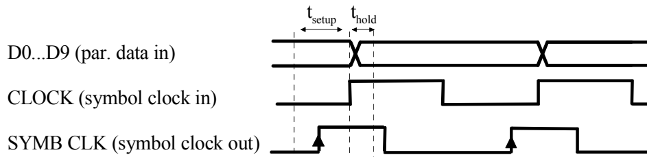
Fig. 4-9 External parallel data with high and low active external symbol clock. The setup time ( t_{\text{setup}} ) and hold time ( t_{\text{hold}} ) can be found in the data sheet.
