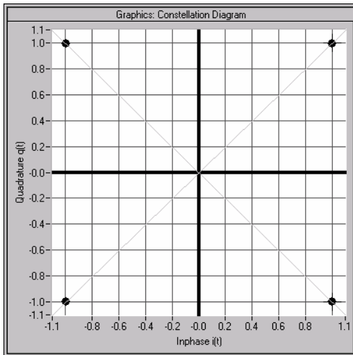
Fig. 4-48 Constellation diagram of a BPSK channel with 0 dB power
