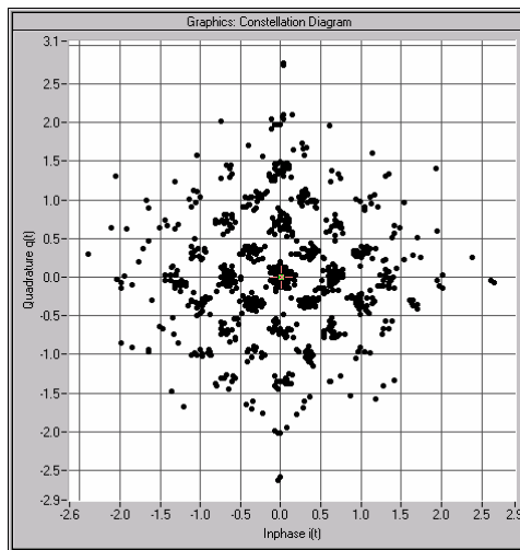
Fig. 4-63 Constellation diagram of the signal without clipping, shows the level mapping
