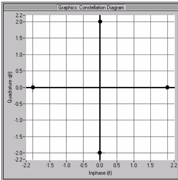
Fig. 4-49 Constellation diagram of a QPSK channel with 0 dB power
