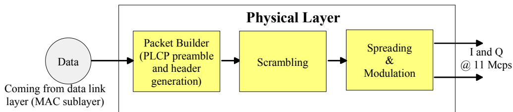
Fig. 4-56 Principle of 802.11b/g signal generation
