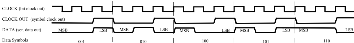
Fig. 4-4 Output signal on the serial data interface and clock output signals on the AUX I/O interface
