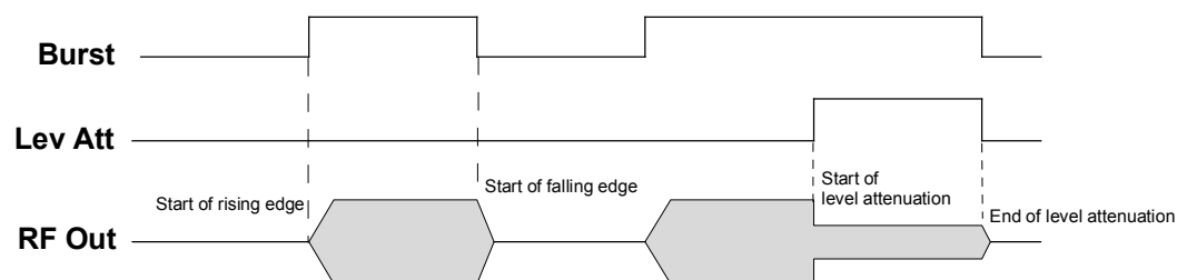
Fig. 4-10 Signal behavior when power ramping is enabled. The Burst Gate signal defines the start of the rising and falling edges of the envelope, and the Lev_Att signal defines the start and end of level attenuation. The level attenuation value is defined in the Power Ramp Control menu.
