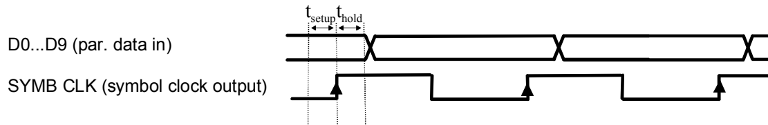
Fig. 4-7 External parallel data, internal clock signal and the clock signal that is output on the AUX I/O interface. The setup time ( t_{\text{setup}} ) and hold time ( t_{\text{hold}} ) can be found in the data sheet.
