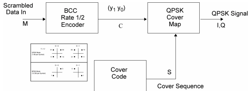
Fig. 4-57 Principle of PBCC modulation
