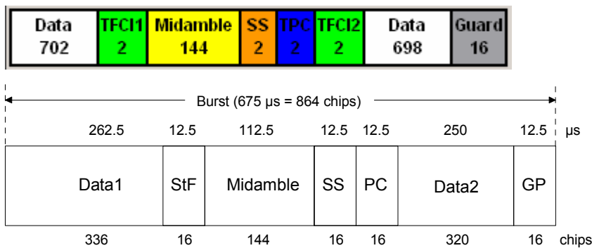
Fig. 4-62 Traffic burst with layer 1 control information
