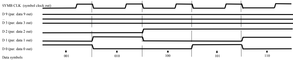
Fig. 4-5 Data and clock output signals on the parallel AUX I/O interface
