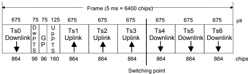
Fig. 4-58 Structure of TD-SCDMA frame
