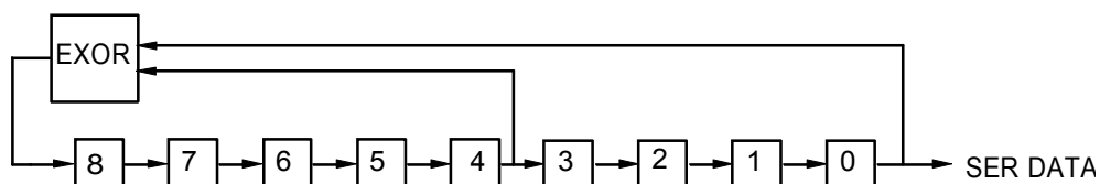
Fig. 4-3 9-bit PRBS generator
