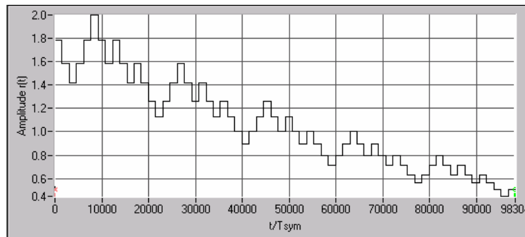
Fig. 4-54 Dynamic change of channel power (continuous)
