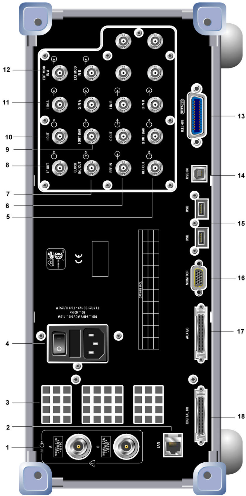
Fig. 1-2 Rear panel view
