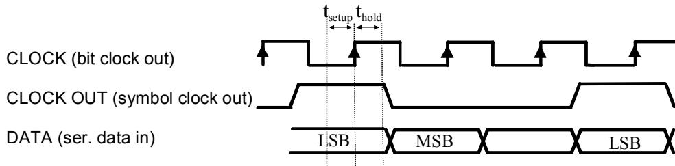
Fig. 4-6 External serial data and the clock signals which are output (bit clock and symbol clock). The setup time ( t_{setup} ) and hold time ( t_{hold} ) can be found in the data sheet.
